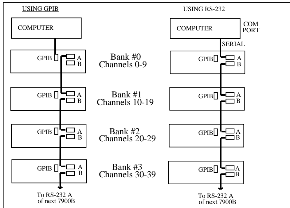
FIGURE 7-1 FOM-7900B Stacked System
