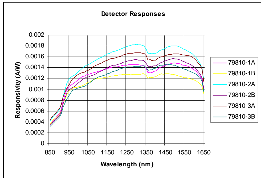
FIGURE 5-1 Sample Detector Response
